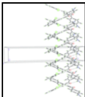
Fig. 3. The crystal packing of (I), viewed down the c -axis, showing 1-D zigzag chains along the b -axis.
